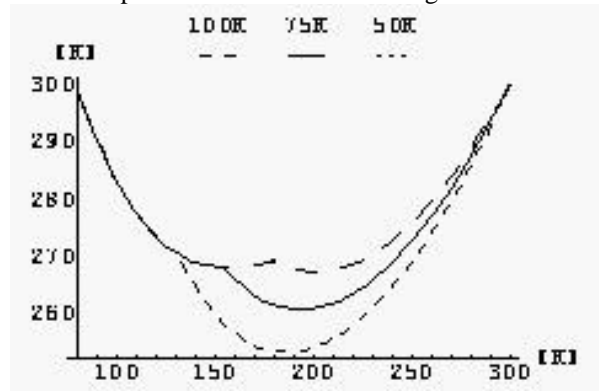
Figure 6 Warm end helium return temperature versus cold helium return temperature as for the solution for Figure 1B
