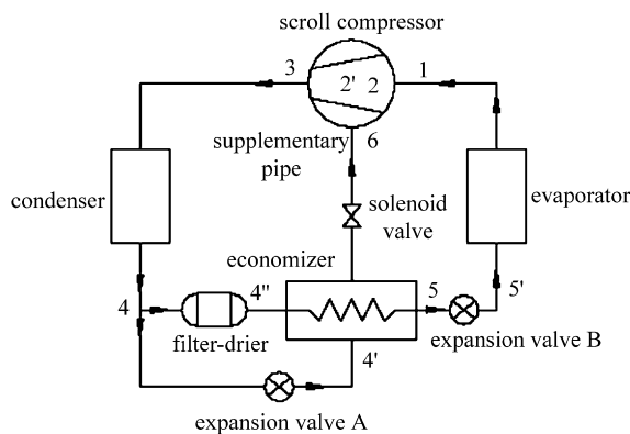
Fig. 4. Schematic of a heat pump system with economizer coupled with scroll compressor drawn by Ma and Li [53].
