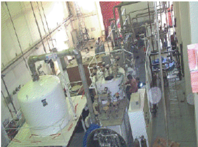
Helium cold-box and MCD (2500 L)
