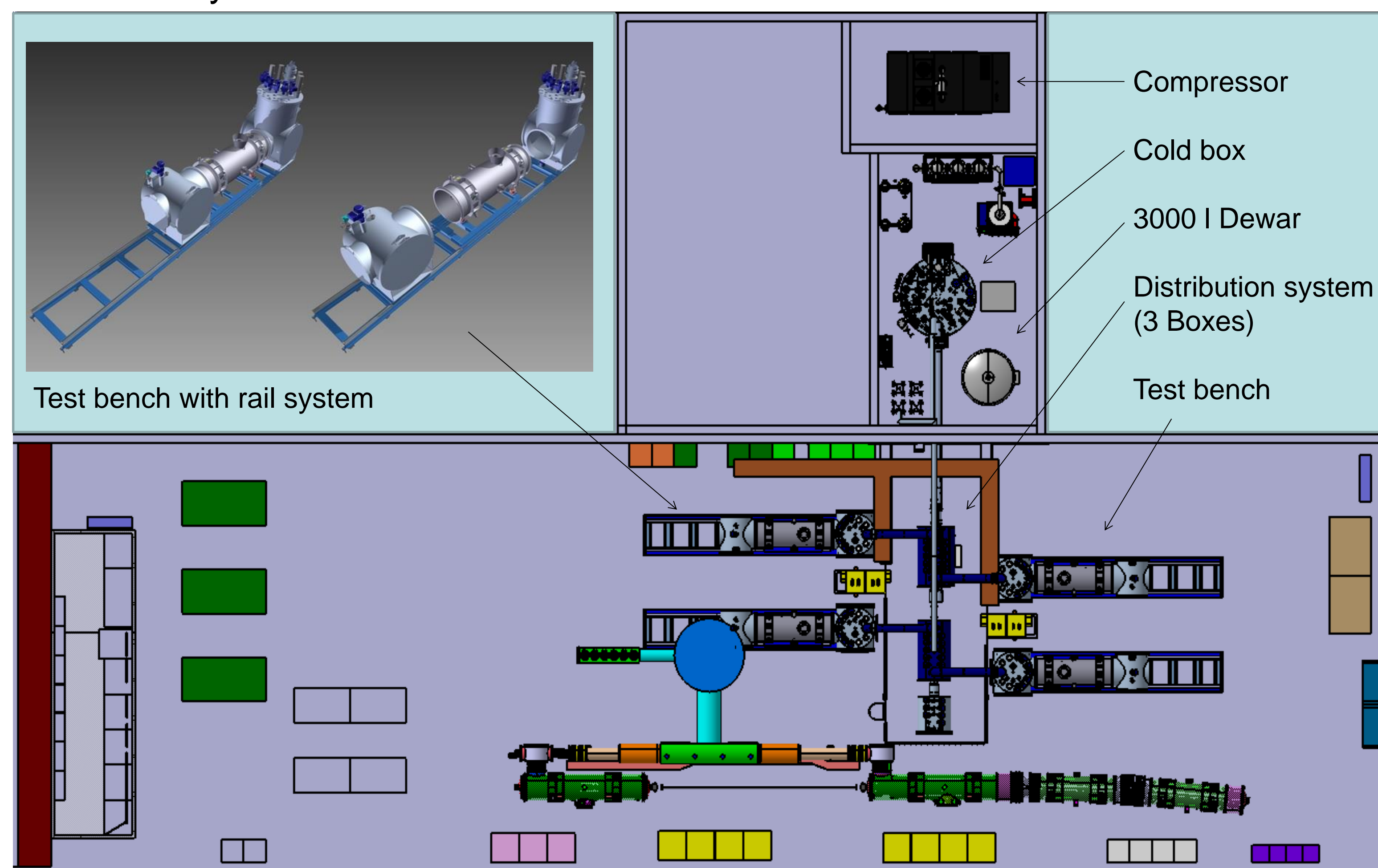
Installation overview
