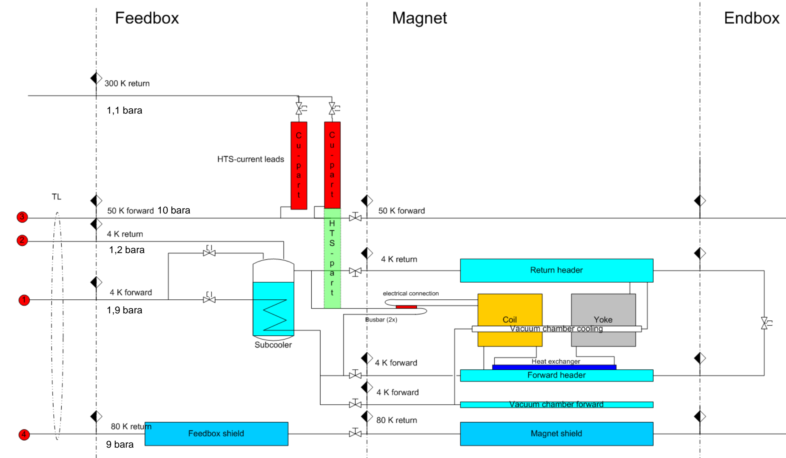
Cooling scheme of the Feed- and Endbox with magnet
